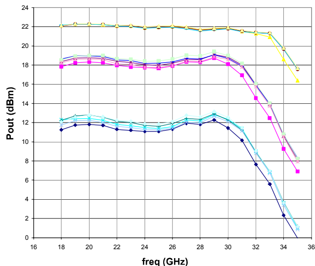
XB1004-BD: Pout vs. freq at -10, -3 and 7dBm
