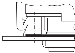
Front mounted connector with FRH1/5 and F-GK1/5
