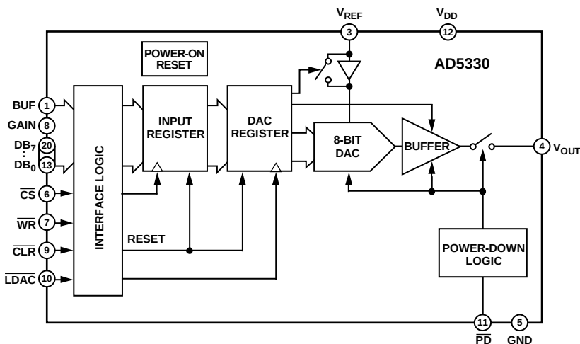
Figure 1. AD5330
