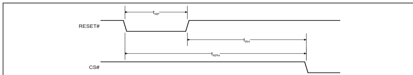
Figure 24 Hardware reset timing diagram
