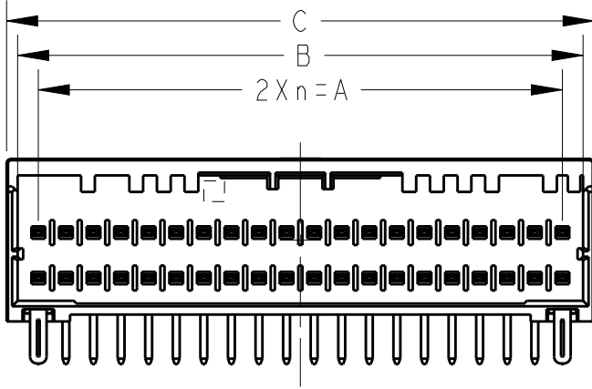
40POS(X-KEY): 1-2271888-0
