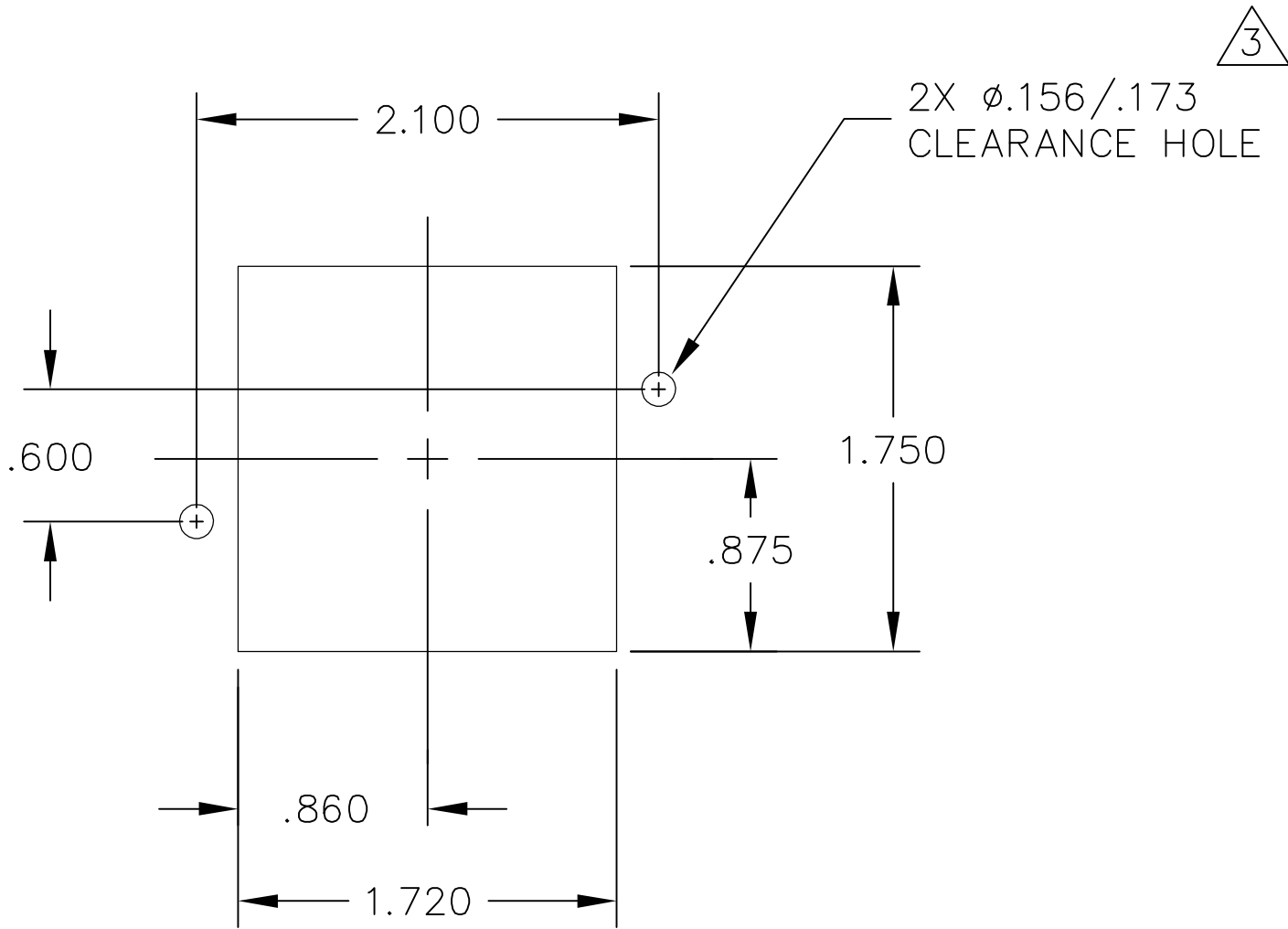
PIN PANEL MOUNT CUTOUT
