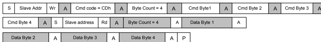
Figure 7-5 CSR Read Operation Using SMBus Block Read – Block Write Process Call
