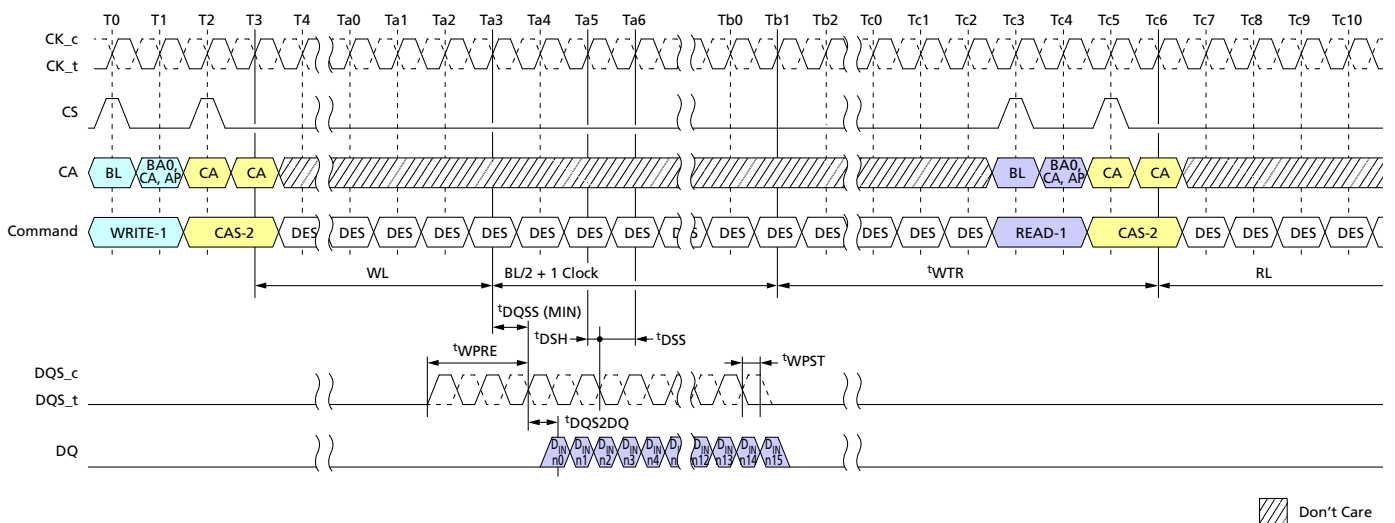
Figure 26: Burst Write Followed by Burst Read
