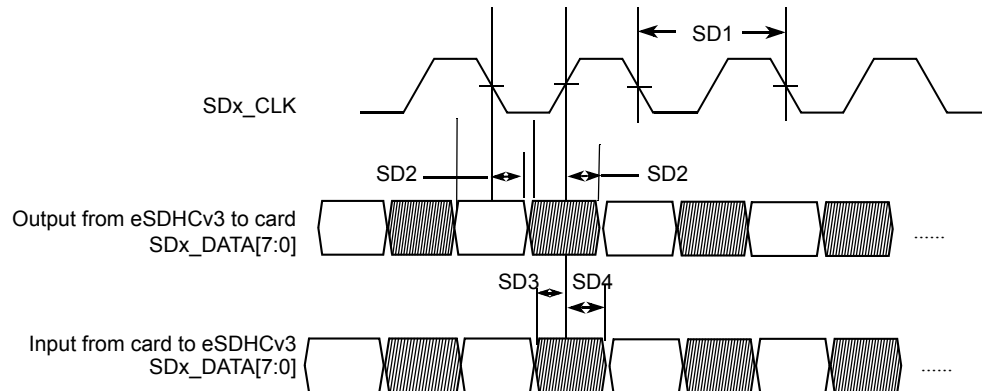
Figure 38. eMMC4.4/4.41 Timing
