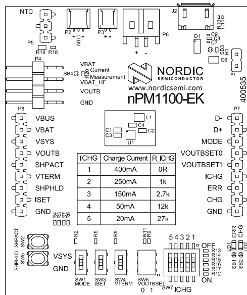
Figure 2: nPM1100 EK front view
