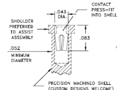
#30 CONTACT FOR .015"-.025" DIAMETER PINS ( \delta = .005 ) 4-FINGER, GROUP C (See page 248)
