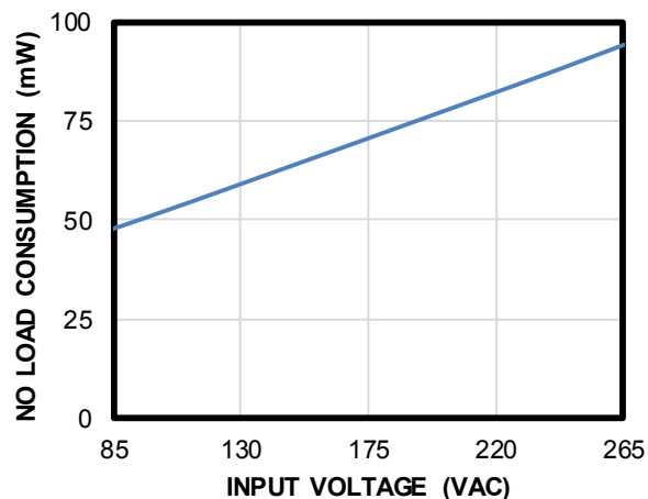
No-Load Consumption
