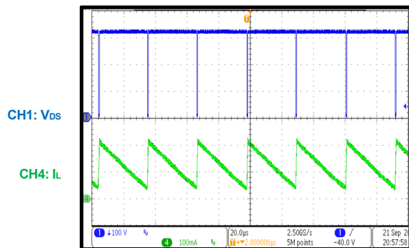
Steady State
