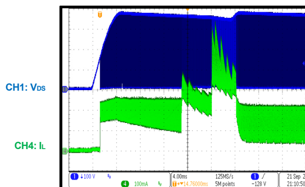
Start-Up
