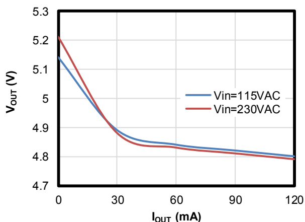
Load Regulation
