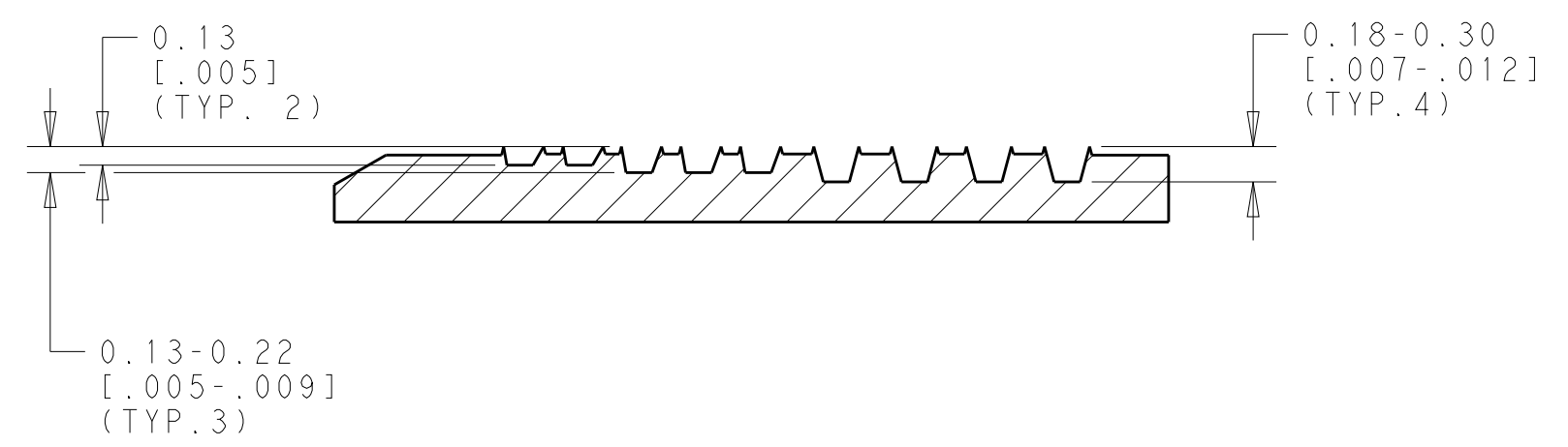
SECTION A - A SCALE 20:1
