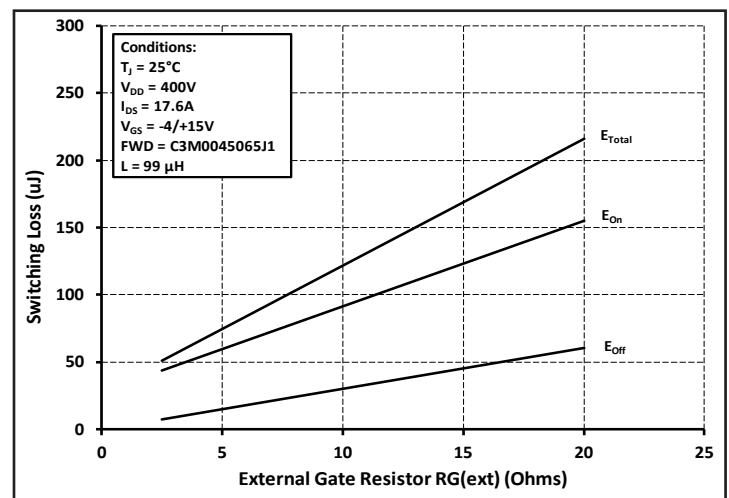
Figure 24. Clamped Inductive Switching Energy vs. R_{G(\text{ext})}
