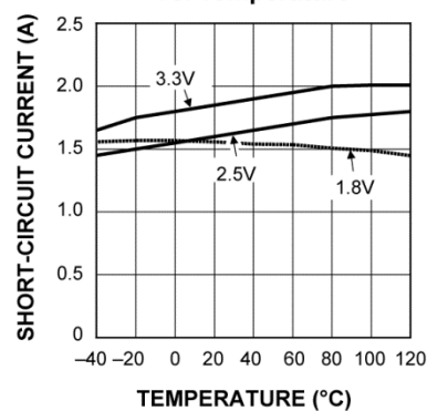
Short Circuit vs. Temperature
