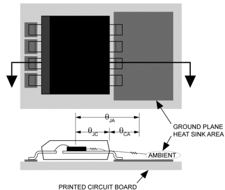
Figure 3. Thermal Resistance
