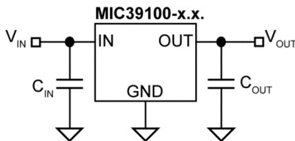
Figure 1. Capacitor Requirements
