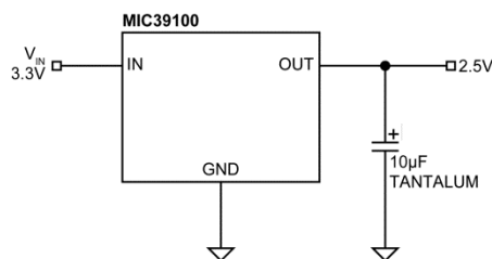
2.5V/1A Regulator
