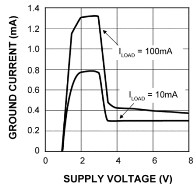
Ground Current vs. Supply Voltage (3.3V)
