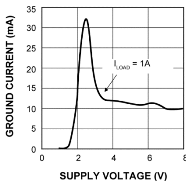
Ground Current vs. Supply Voltage (2.5V)
