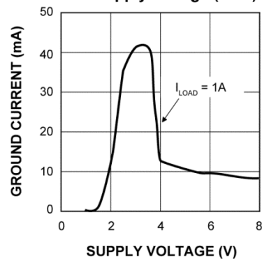
Ground Current vs. Supply Voltage (3.3V)
