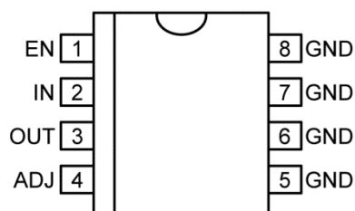
MIC39102 Adjustable SOIC-8 (M) (Top View)
