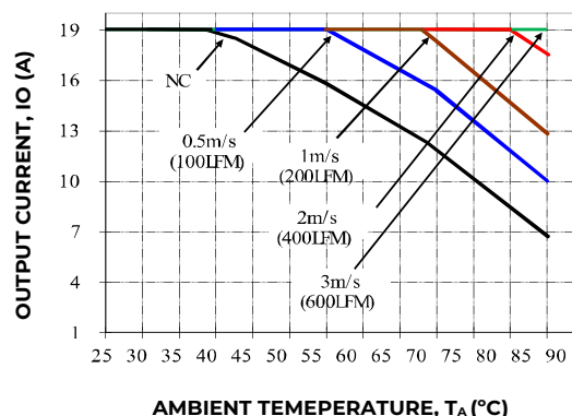
Figure 19. Output Current Derating for the Module with Heatplate; Airflow in the Transverse Direction from V_{out}(+) to V_{out}(-) ; V_{IN} = 24V , V_O = 12V .
