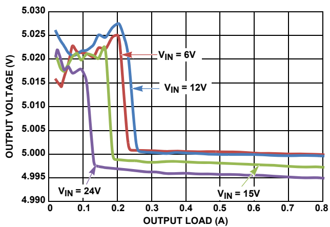
FIGURE 14. V_{OUT} REGULATION vs LOAD, PFM, V_{OUT} = 5\text{V} , L_1 = 30\mu\text{H}
