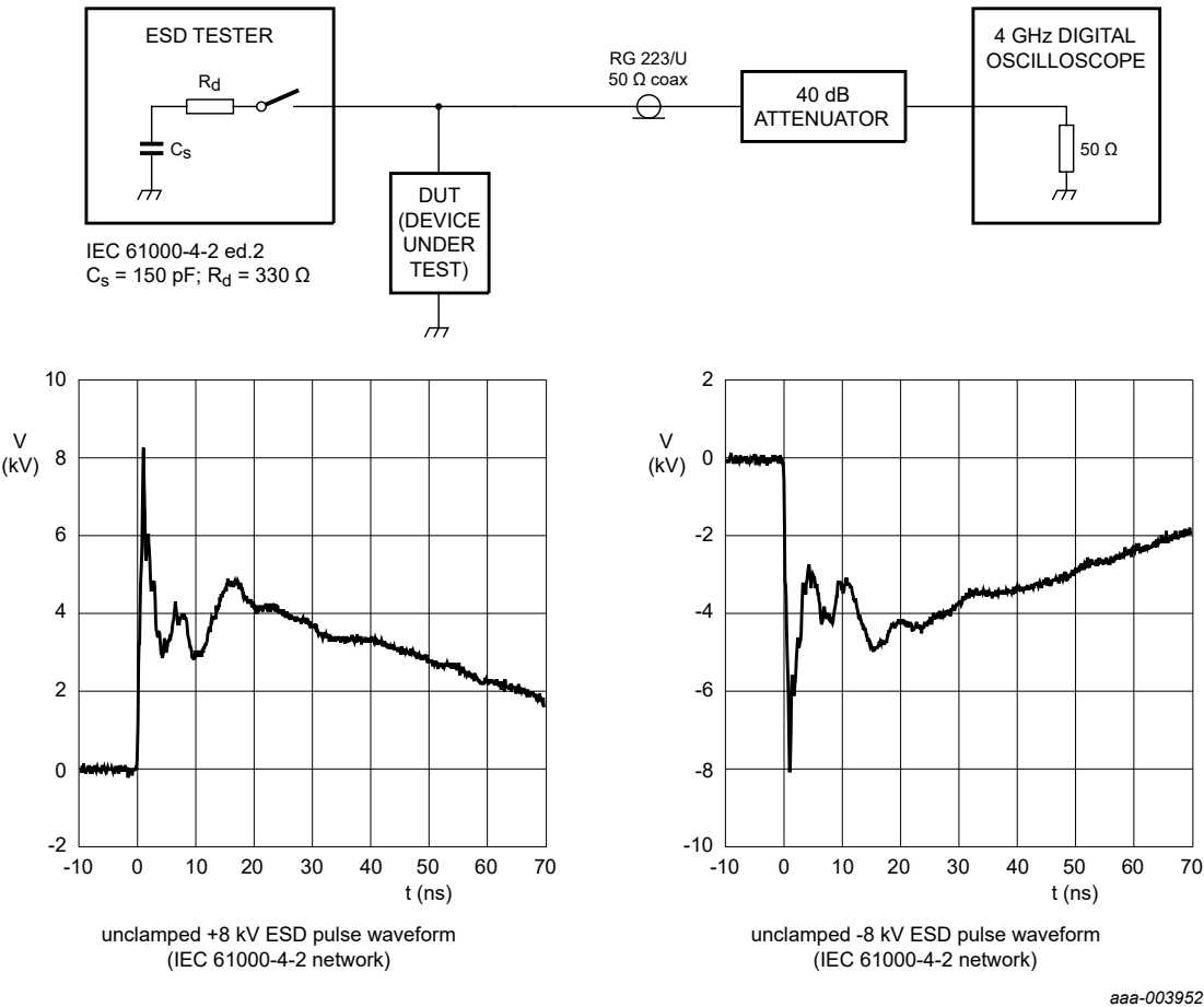
Fig. 11. ESD clamping test setup and waveforms
