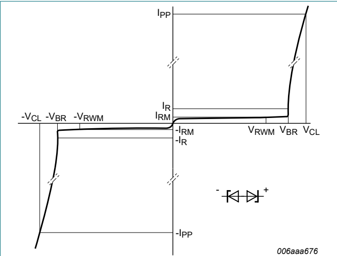
Fig. 4. V-I characteristics for a bidirectional ESD protection diode
