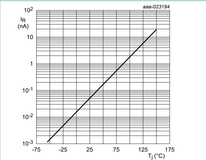
Fig. 5. Relative variation of reverse leakage current as a function of ambient temperature; typical values
