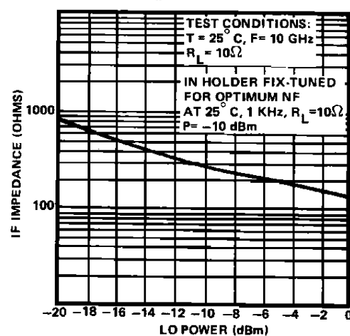
Z_{IF} vs POWER
