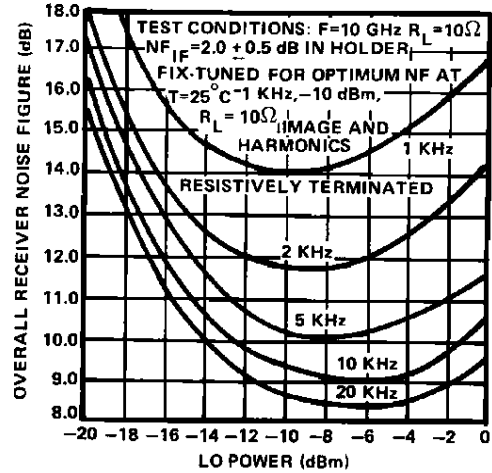
SINGLE SIDEBAND NOISE FIGURE vs POWER
