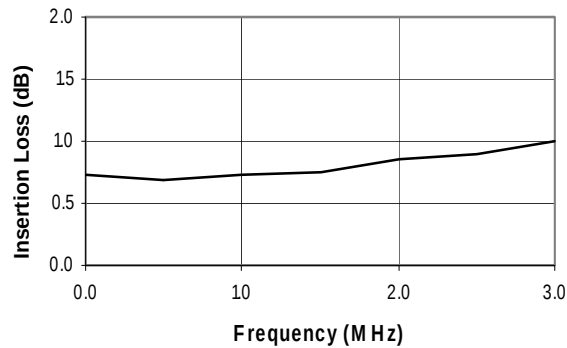
Insertion Loss
