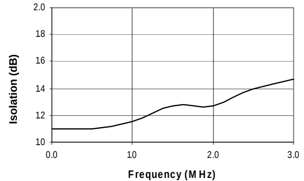
Isolation
