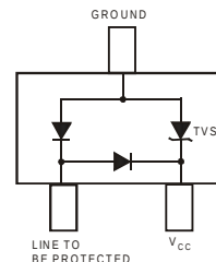
Device Schematic
