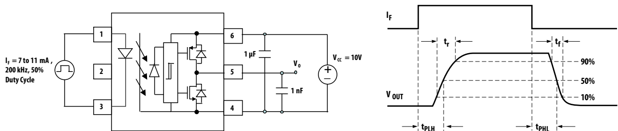
Figure 14: t_r and t_f Test Circuit and Waveforms
