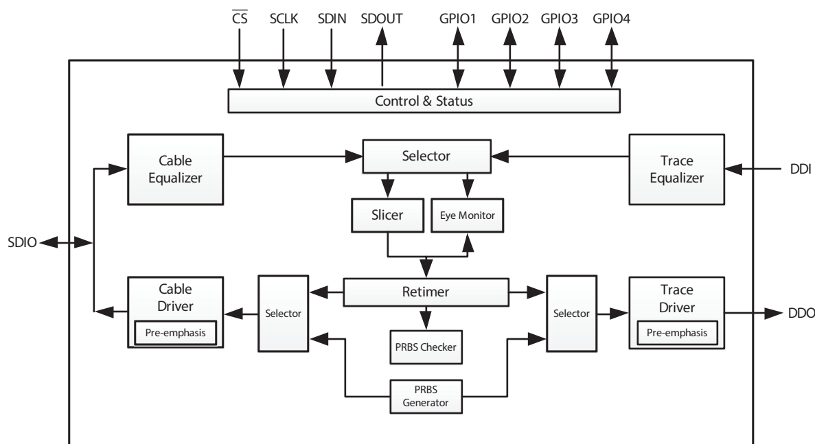
GS12090 Functional Block Diagram
