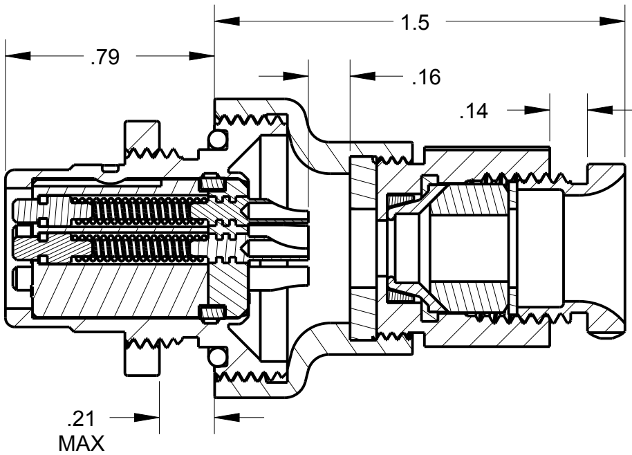
SECTION Z-Z
