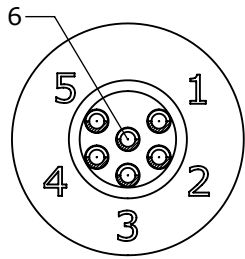
WIRING END ASSY: 7282-6PG-3ES
