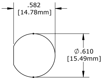
RECOMMENDED PANEL CUT-OUT TOLERANCE: ±.003
