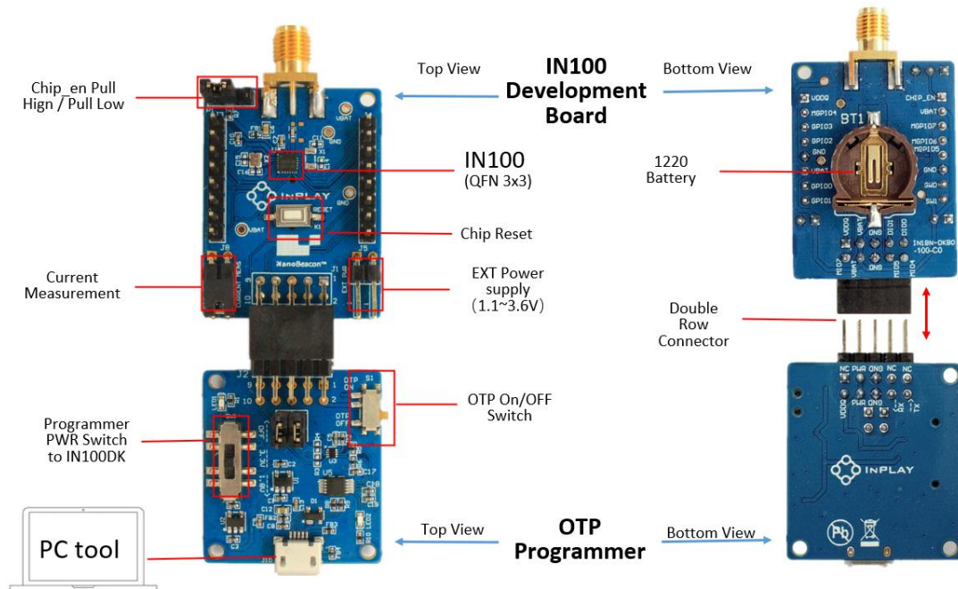
Figure 3 NanoBeacon development kit (front and back view)
