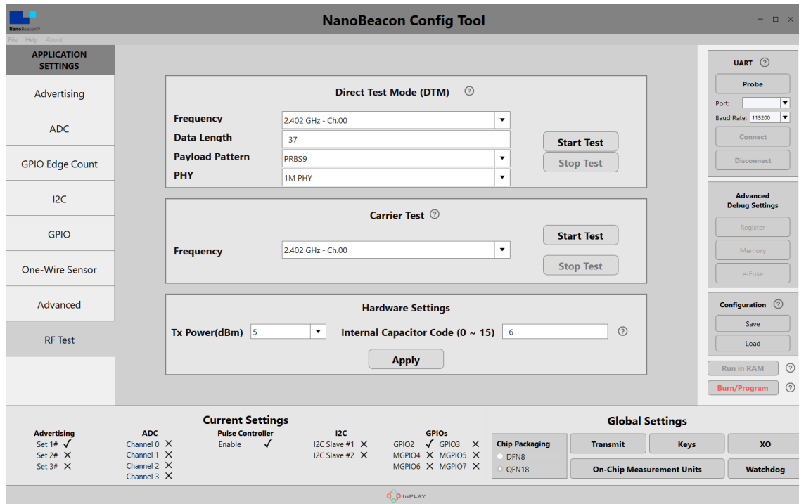
Figure 46 RF test configuration
