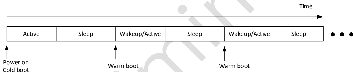
Figure 42 IN100 states
