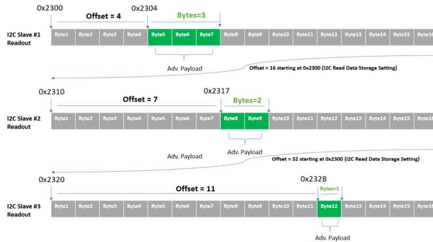
Figure 11 I2C read data as adv. payload
