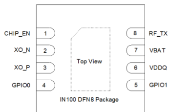
Figure 47 DFN8 package
