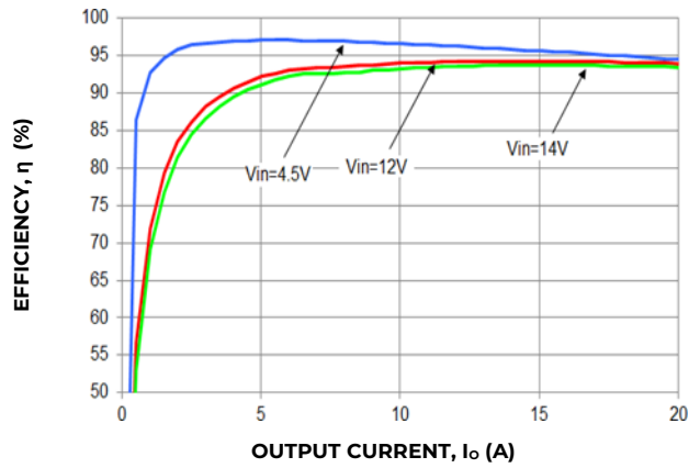
Figure 25. Converter Efficiency verses output current
