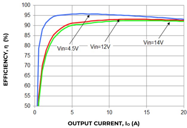
Figure 19. Converter Efficiency verses output current
