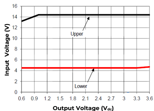
Figure 35. Output Voltage vs. Input Voltage Set Point Area plot showing limits where the output voltage can be set for different input voltages.
