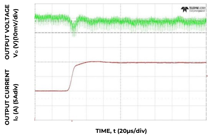
Figure 4. Transient Response to Dynamic Load Change from 50% to 100% at 12V in , C out = 7x47μF + 9x330μF, C Tune =15nF, R Tune =300
