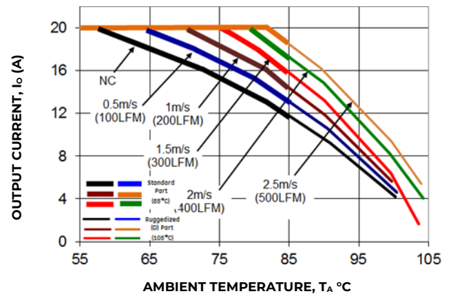
Figure 20. Derating Output Current verses Ambient Temperature and Airflow.
