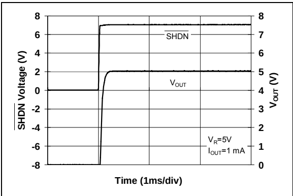
FIGURE 2-41: SHDN Response.
