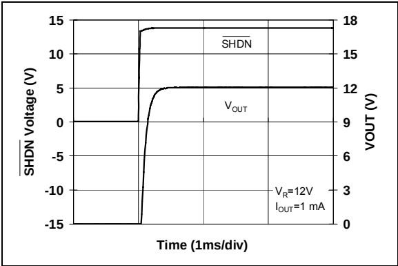
FIGURE 2-42: SHDN Response.
