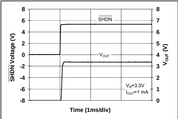
FIGURE 2-40: SHDN Response.
