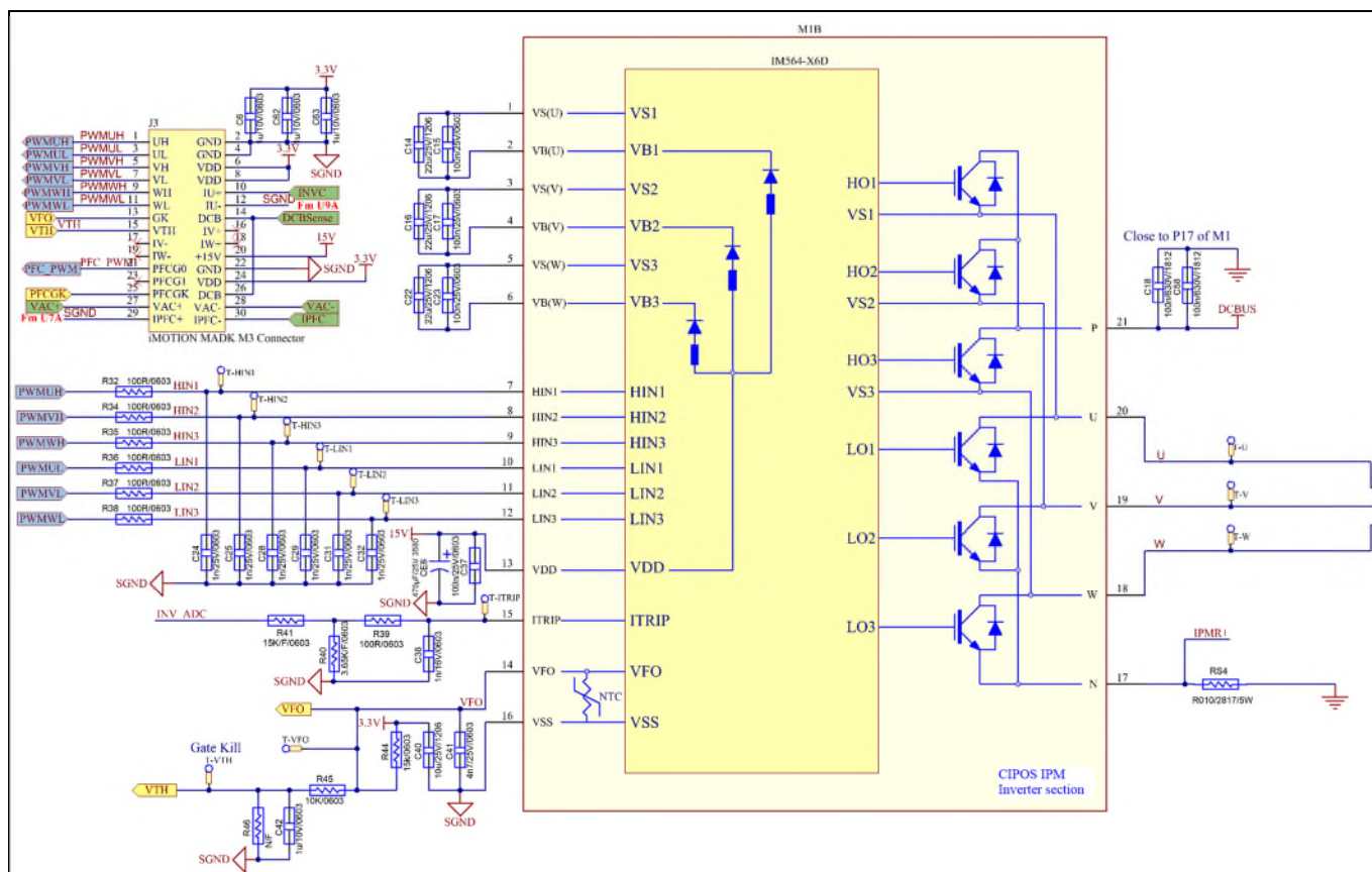
Figure 34 Inverter section schematics for EVAL-M3- IM564
