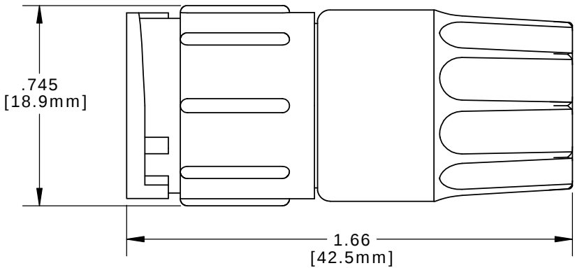
ASSEMBLED VIEW
