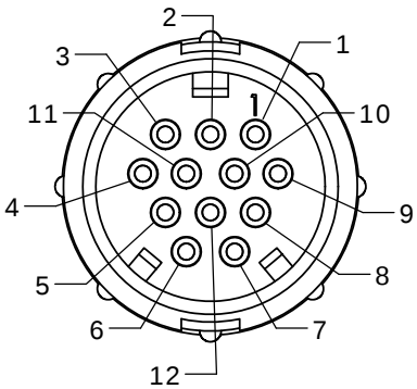
FACE VIEW W5280-12PG-3XX
