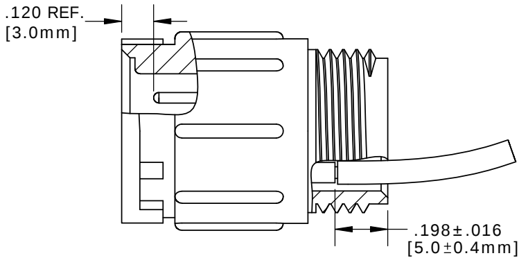
CONTACT INSERTION VIEW
