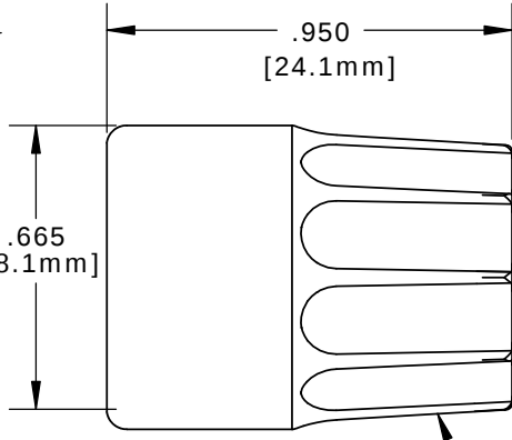
SLEEVE MAT'L: THERMOPLASTIC, BLACK
