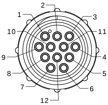
WIRE VIEW
