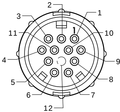
FACE VIEW W5280-11PG-3XX
