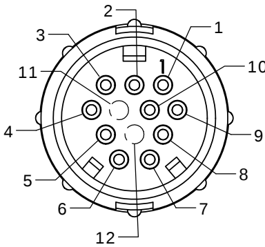
FACE VIEW W5280-10PG-3XX
