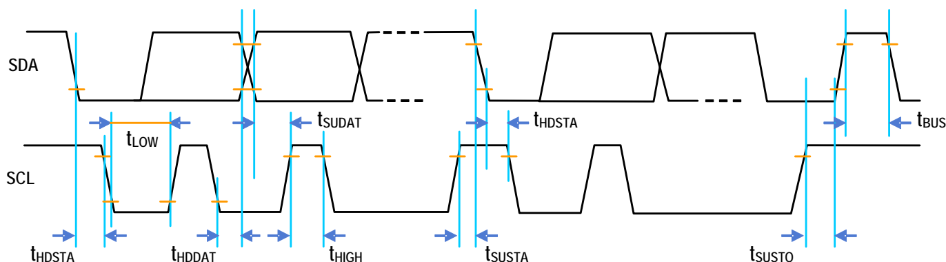
Figure 7. Timing Diagram
