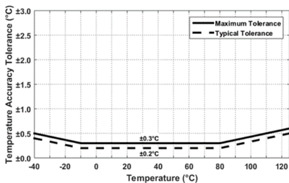
Figure 5. HS4001 Temperature Sensor Accuracy Tolerance
