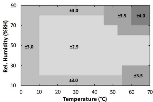
Figure 4. HS4003 RH Accuracy over Temperature
