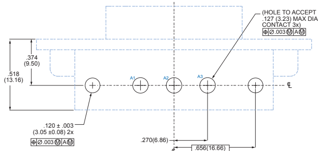
2-3P3 3 #8
