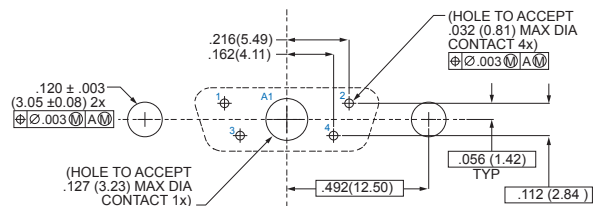
1-5P1 1 #8, 4 #20
