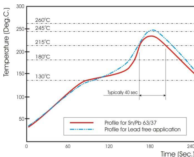
Fig 3. Infrared soldering profile for Chip Resistors
