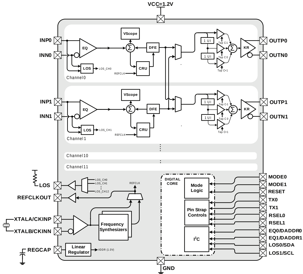
Figure 1. Block Diagram
