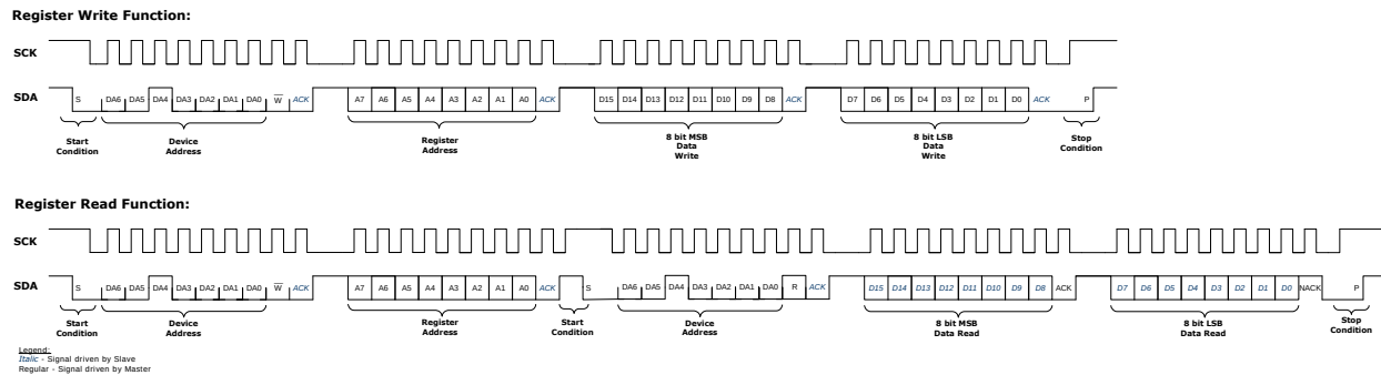
Figure 7. Two-Wire Serial Timing
