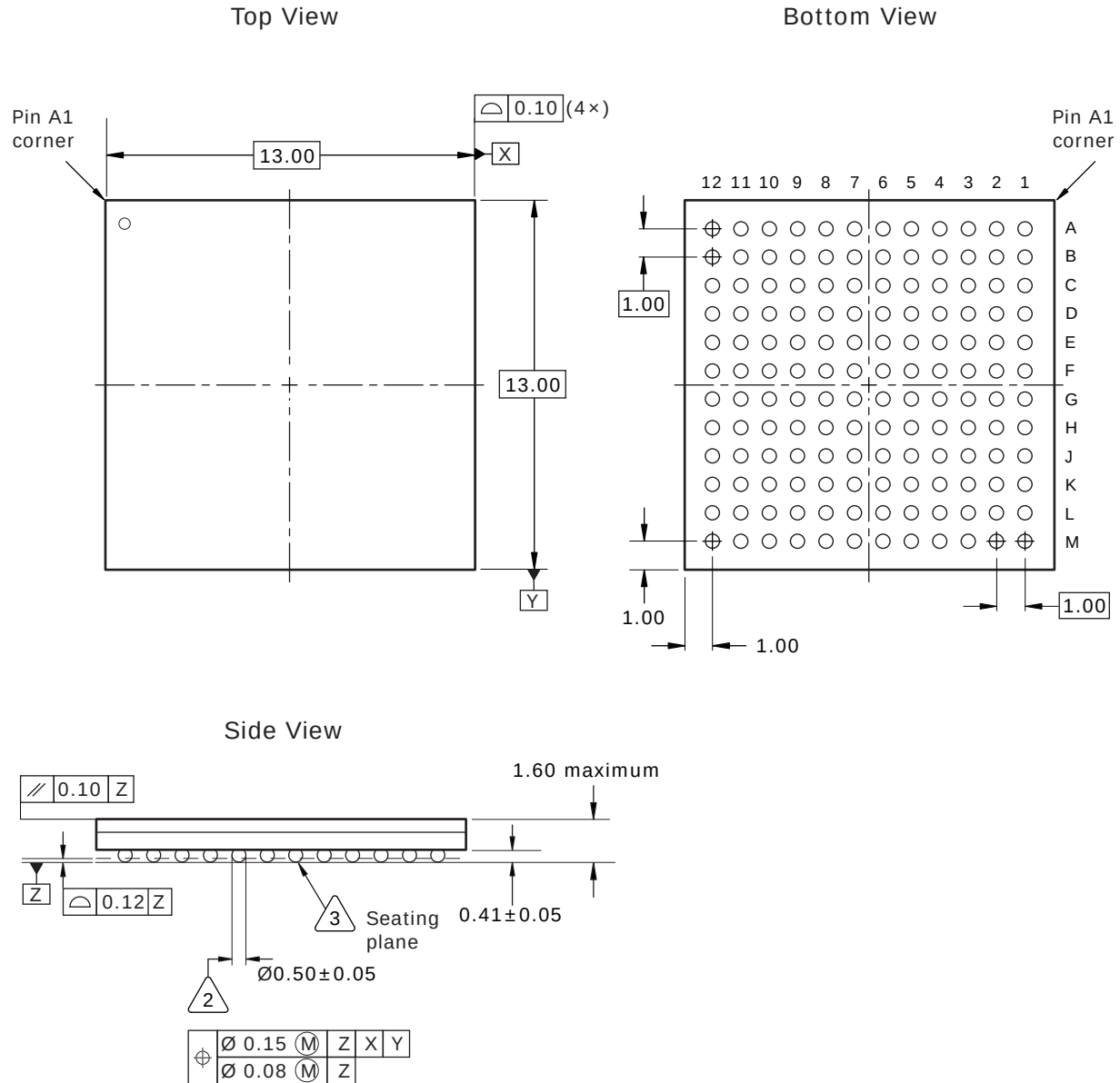
Figure 11. Package Drawing
