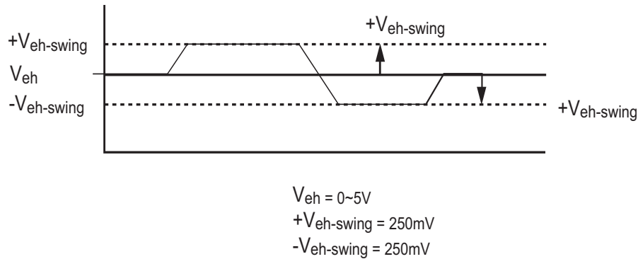
ARC single mode signal output waveform
