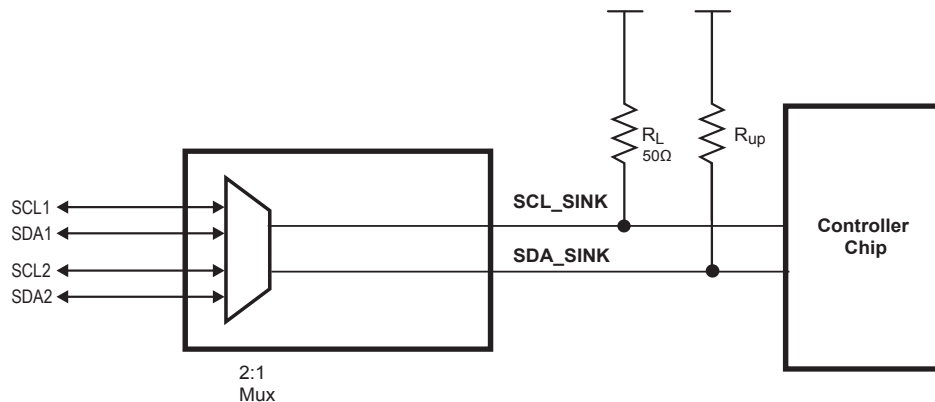
DDC Channel Application Diagram
