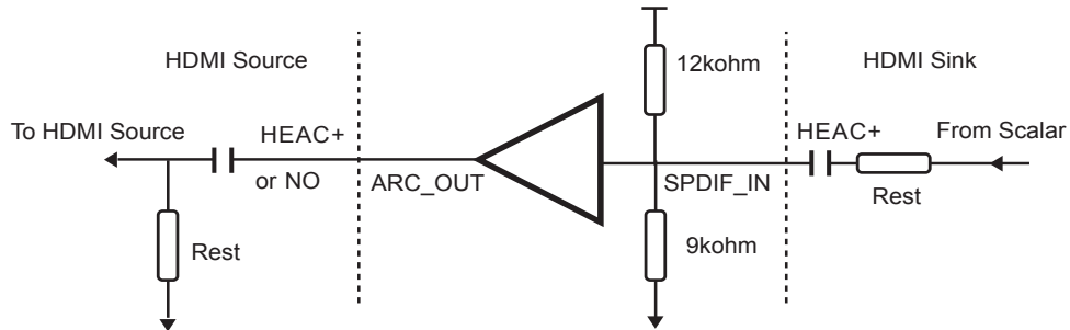
ARC single mode input and output
