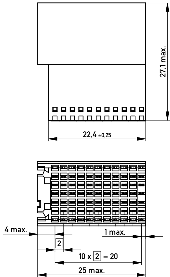
CONTACT LAYOUT
