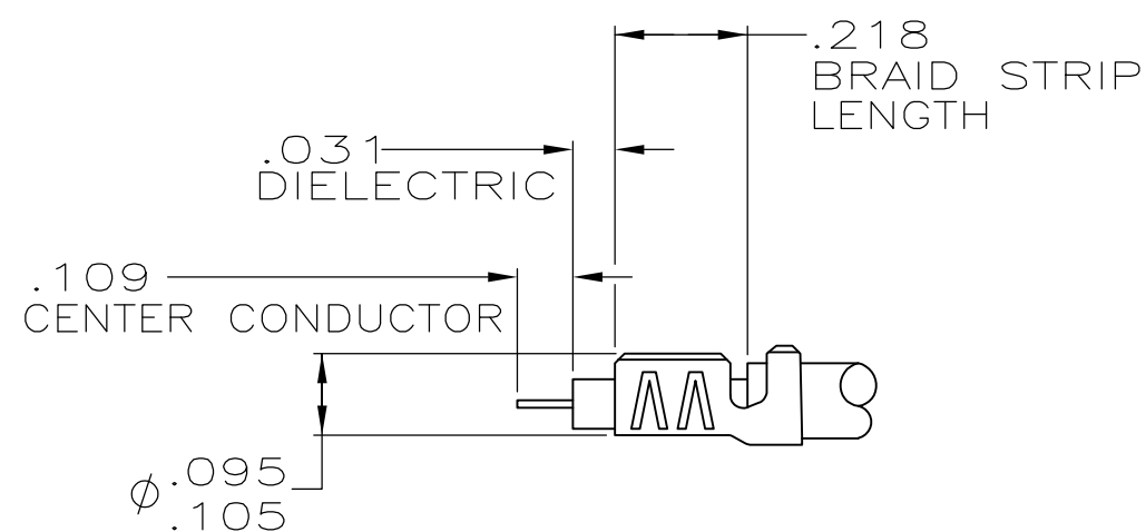
ASSEMBLED VIEW
