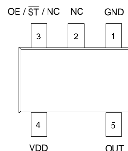
Figure 1. Pin Assignments
