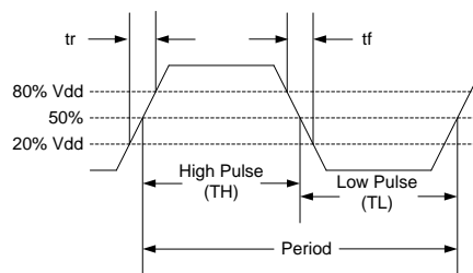
Figure 3. Output Waveform
