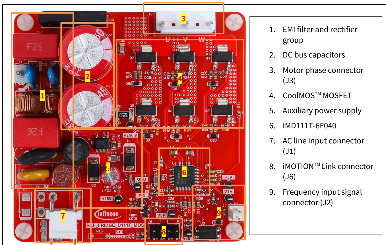
Figure 2 Functional groups on top side of board
