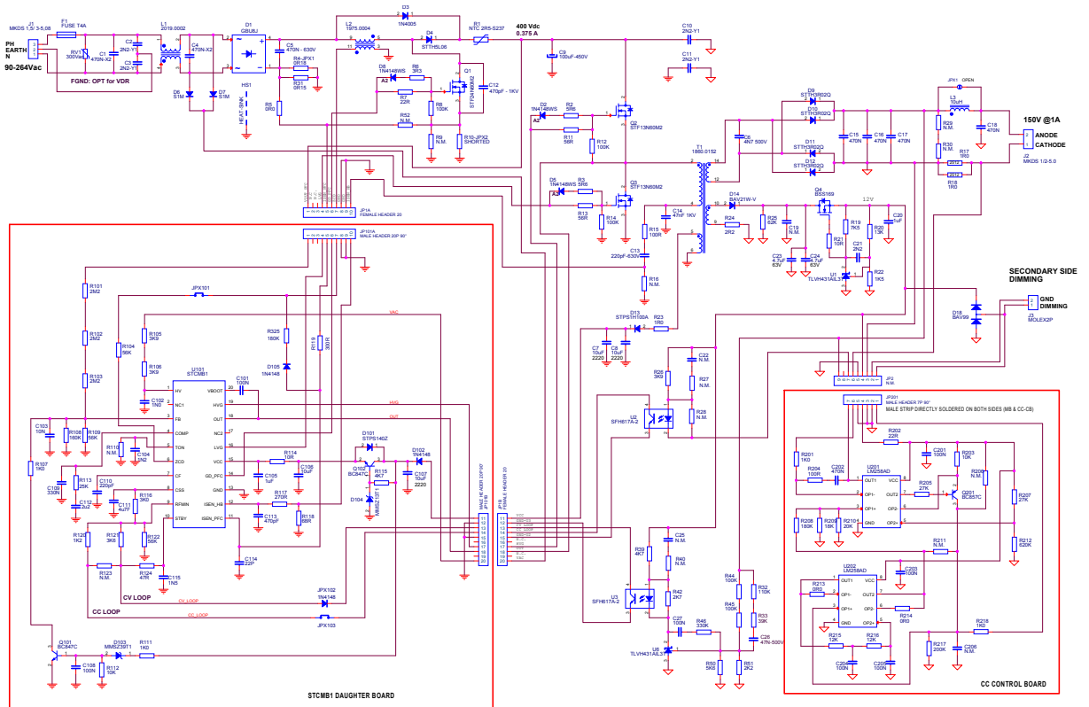
Figure 1. Electrical diagram
