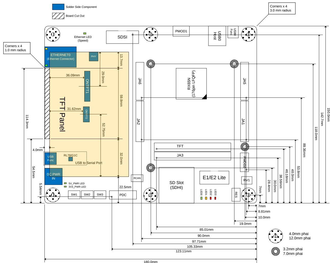
Figure 3-2: Board Dimensions
