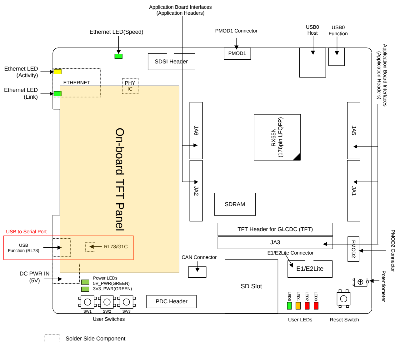
Figure 3-1: Board Layout
