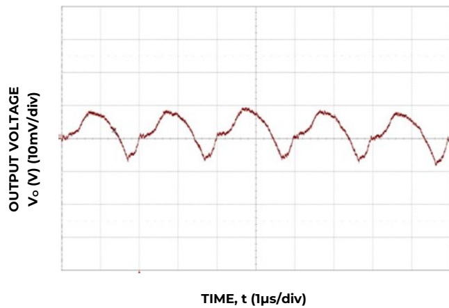
Figure 15. Typical output ripple and noise ( C_o=3 \times 22\mu\text{F} ceramic, V_{IN} = 12\text{V} , I_o = I_{o,max} ).
