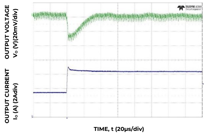
Figure 16. Transient Response to Dynamic Load Change from 50% to 100% at 12V in , C_{out} = 3 \times 47\mu\text{F} + 1 \times 330\mu\text{F} , C_{Tune} = 3.9\text{nF} , R_{Tune} = 300\Omega
