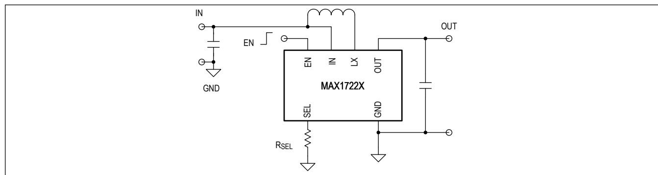
Figure 6. Single R_{\text{SEL}} Resistor Sets the Output Voltage
