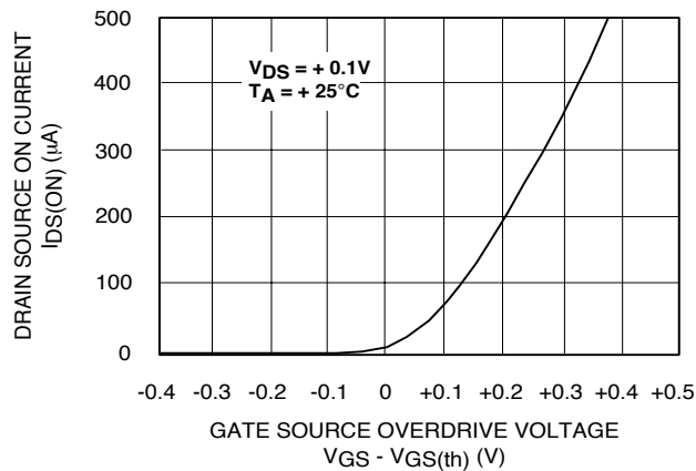
FORWARD TRANSFER CHARACTERISTICS LOW VOLTAGE
