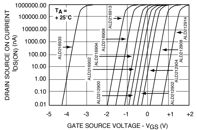
FORWARD TRANSFER CHARACTERISTICS EXPANDED (SUBTHRESHOLD)
