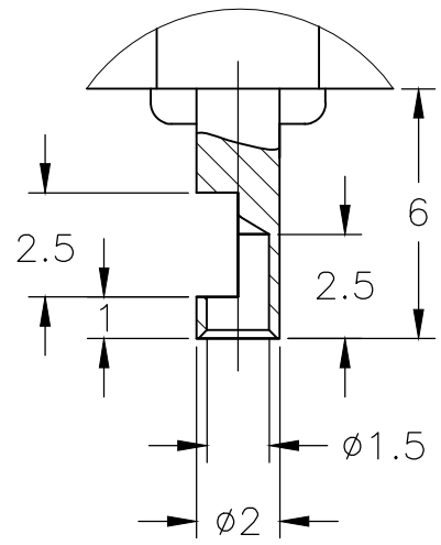
DETAIL 1 SCALE 5:1
