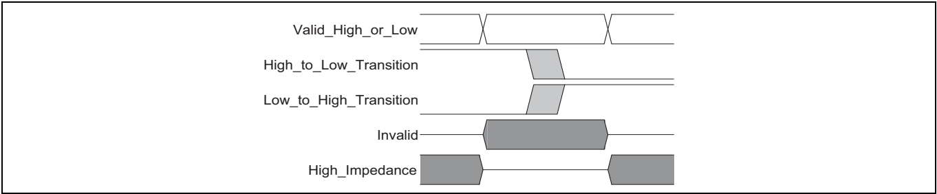
Figure 33 Key to switching waveforms
