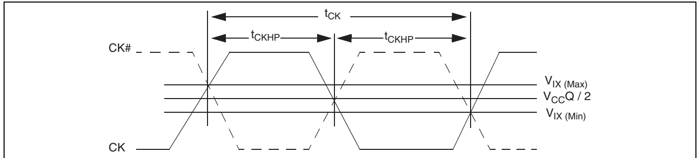
Figure 36 Clock characteristics
