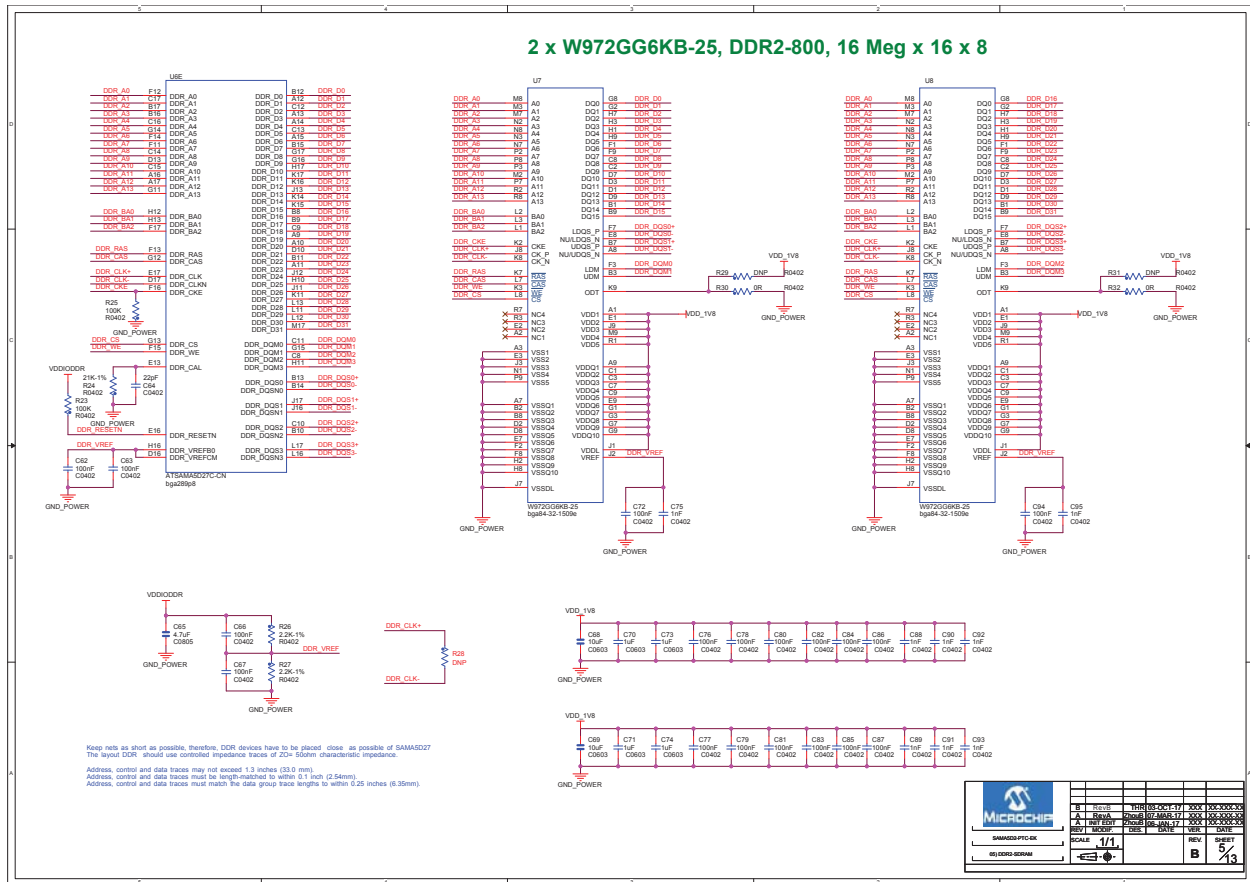
Figure 5-5. DDR2-SDRAM
