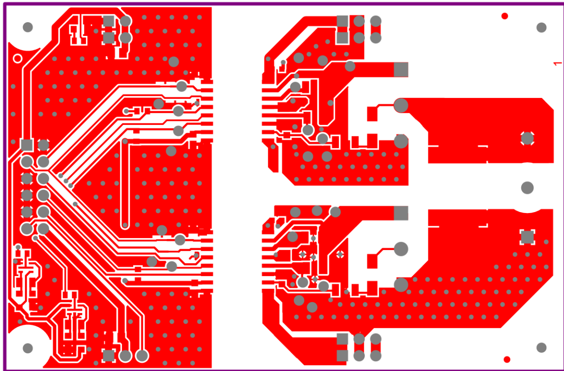
Figure 11 Eval-1ED3321MC12N – PCB top layer view
