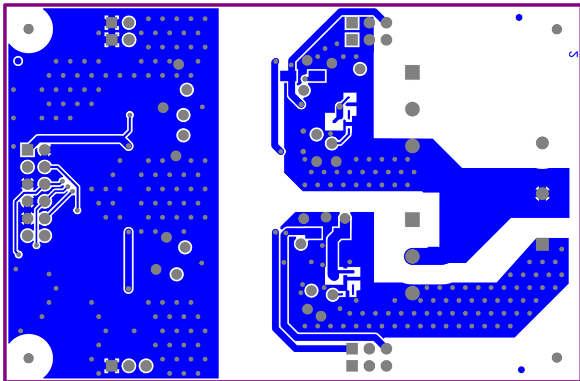
Figure 12 Eval-1ED3321MC12N – PCB bottom layer view
