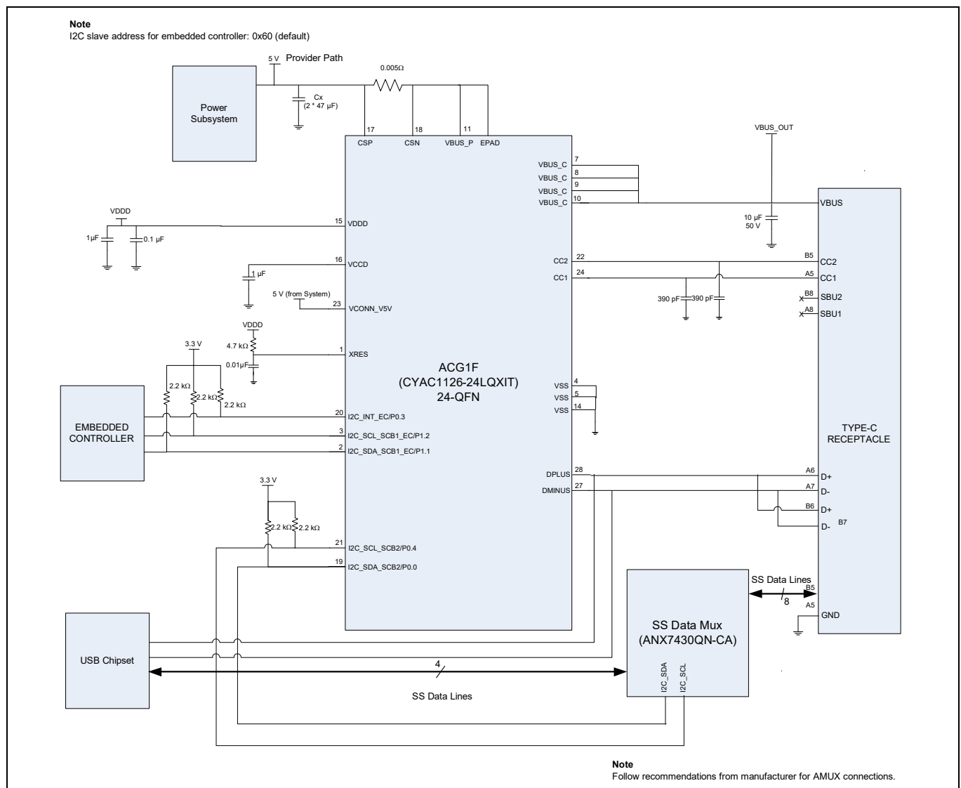
Figure 4-2 ACG1F in Single Port USB Type-C Notebook Application using CYAC1126- 24LQXIT
