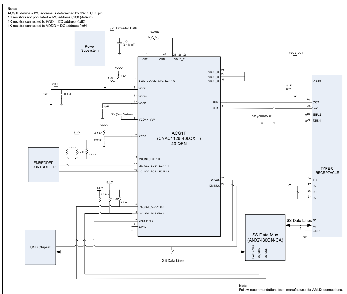
Figure 4-1 ACG1F in Single Port USB Type-C Notebook Application using CYAC1126- 40LQXIT
