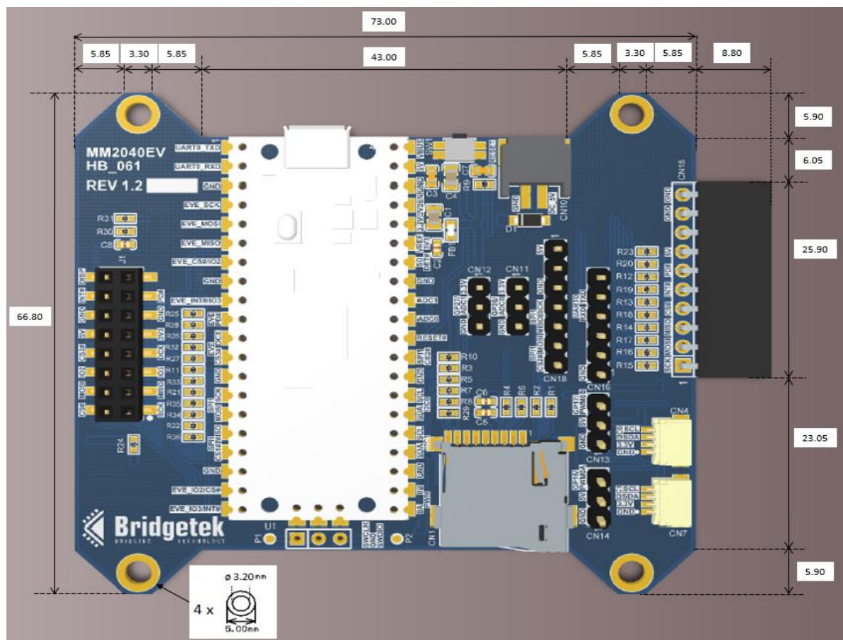
Figure 3 – MM2040EV PICO Adapter Board PCB Dimensions (Top view)
